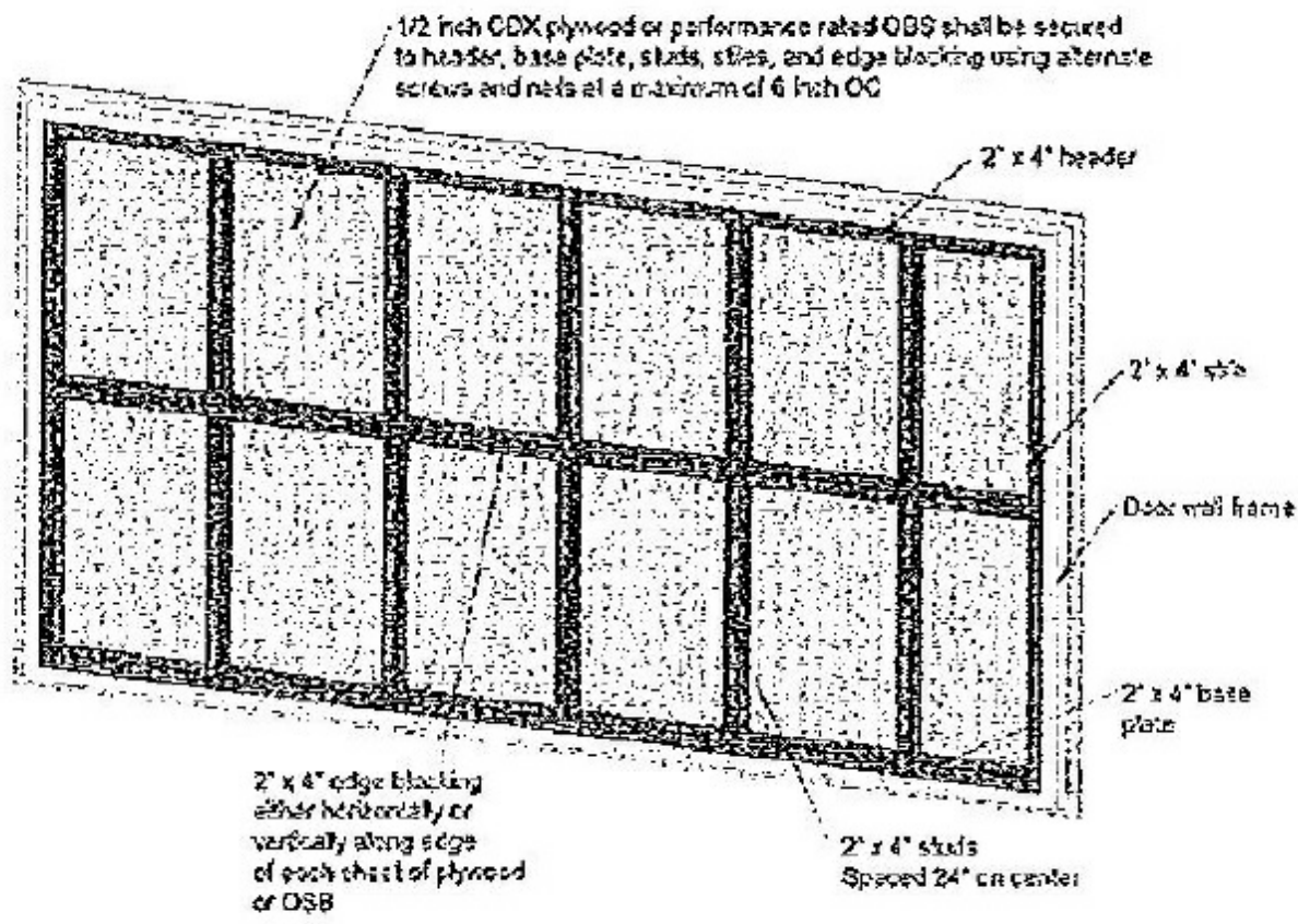
FIGURE A103.1(2) BOARDING OF DOOR WALL
