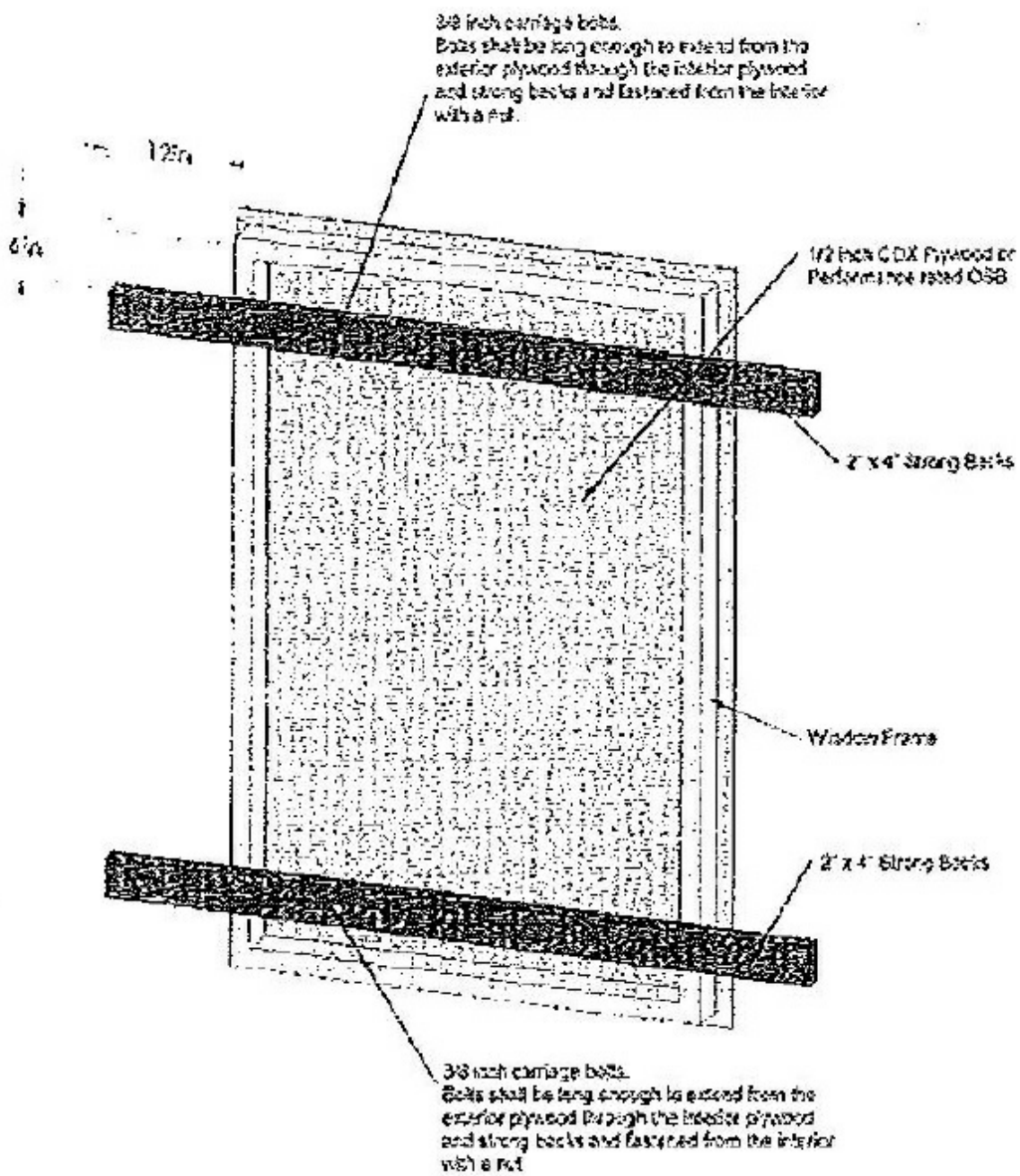
FIGURE A103.1(1) BOARDING OF DOOR OR WINDOW
